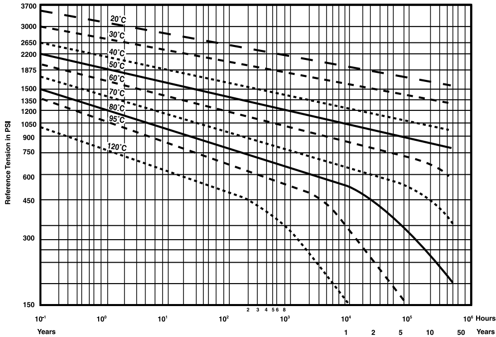
Durability PVDF
