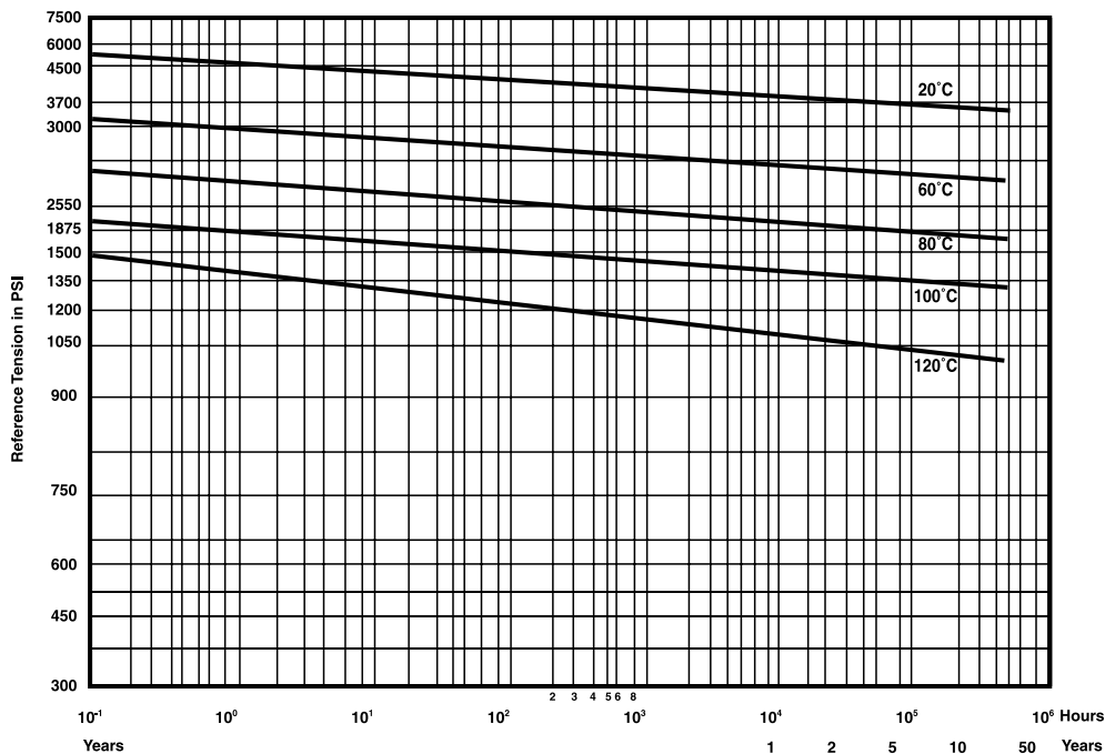
Durability PVDF
