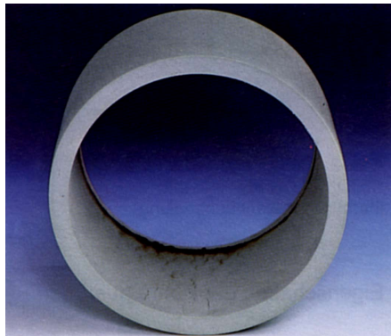
Fig. 3 PP Pipe, Standard Quality After Chromic Acid Test.
