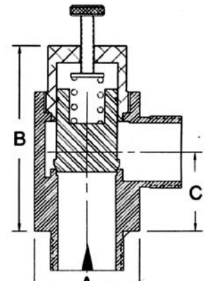
3.00" VALVE STYLE
